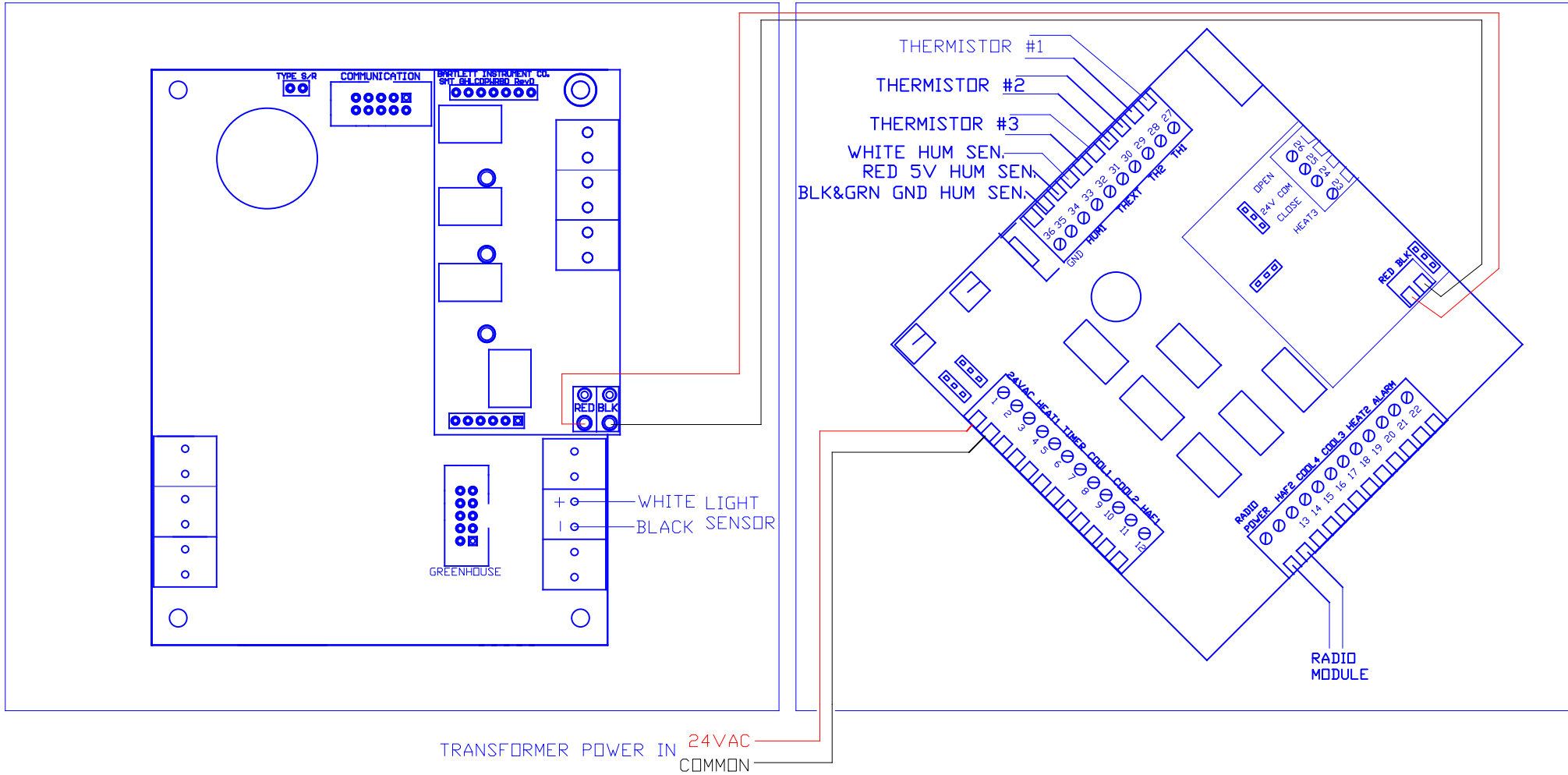
CLIMATEBOSS ENCLOSURE TOP/LID NEGATIVE
